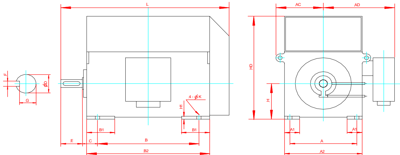
YKK SERIES MOTOR OVERALL AND MOUNTING DIMENSIONS
